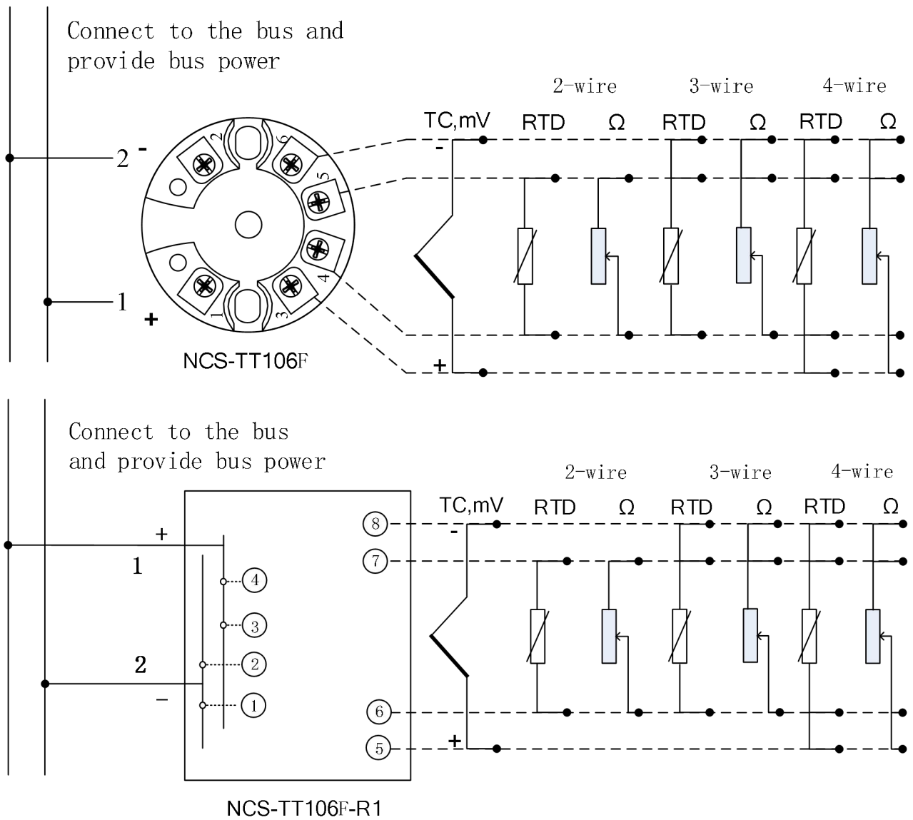
Figure 2.3 Wiring
