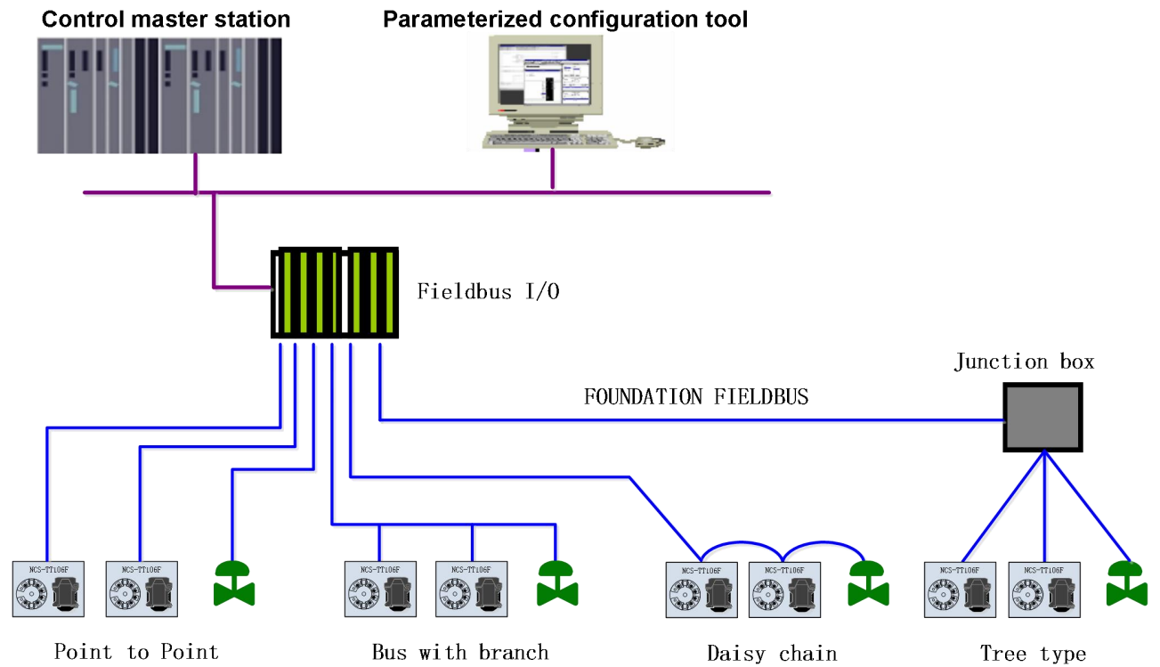
Figure 3.1 Foundation Fieldbus network topology
